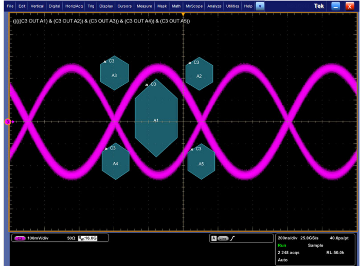
Eye Diagram triggering using optional Visual Trigger.
