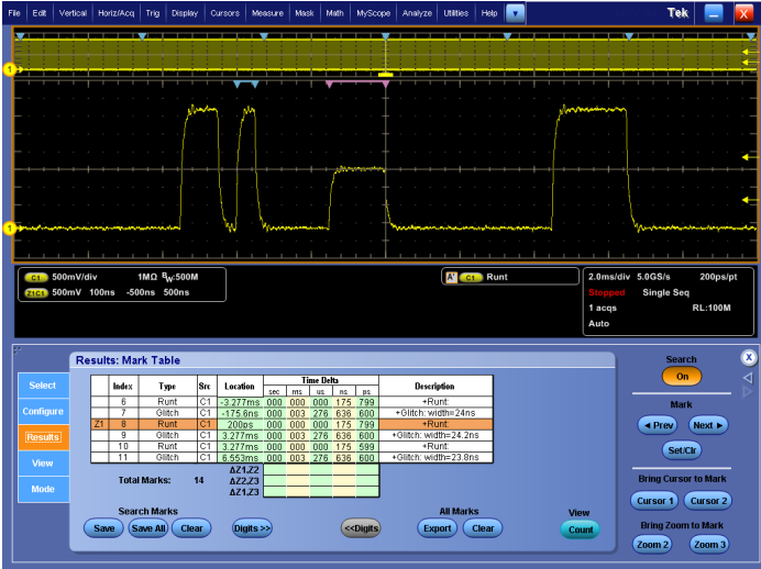
Search – Results of an advanced search for a runt pulse or a narrow glitch within a long waveform record. Each instance of the runt or glitch is automatically marked for easy reference.
