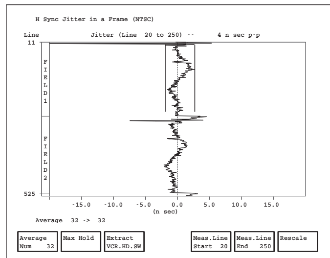
H_Jitter.
