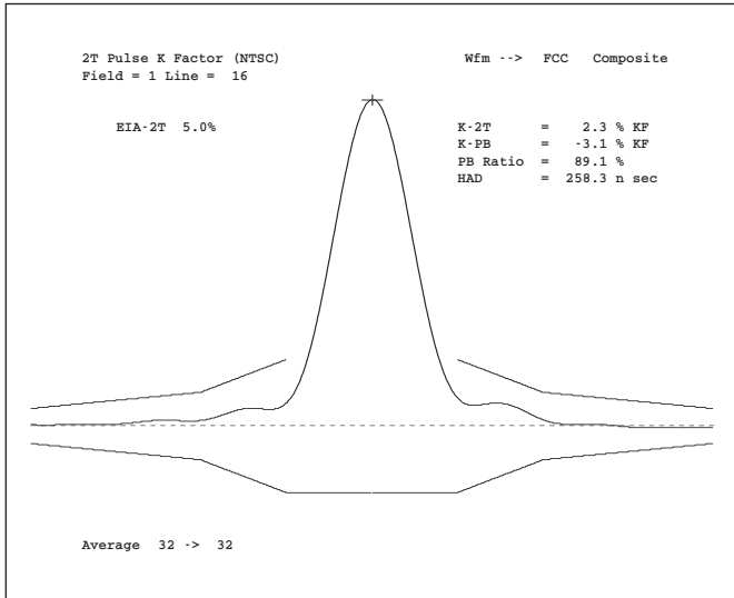
K-factor measurement.
